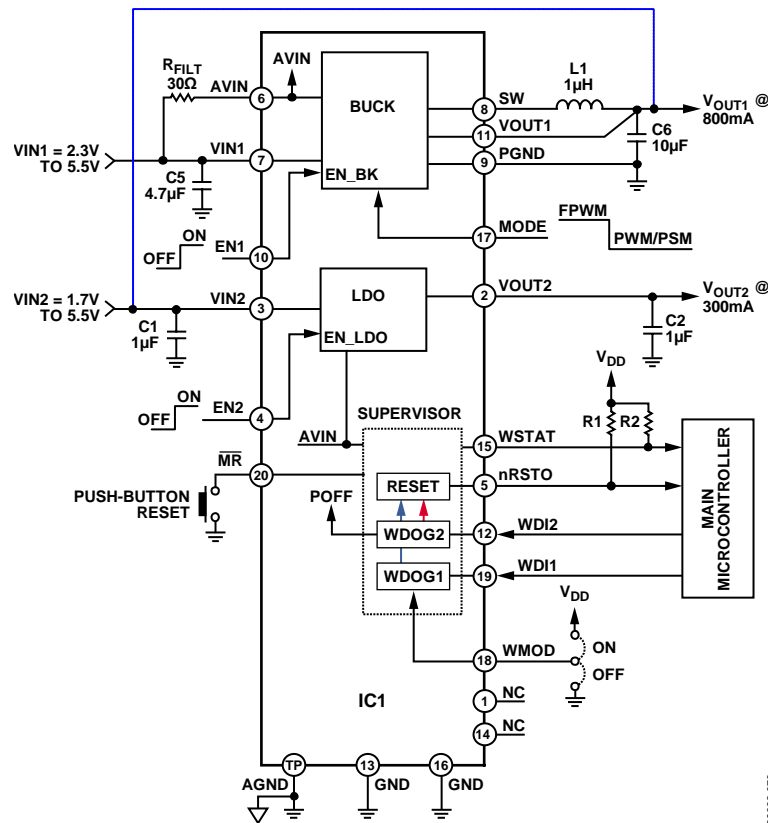
Figure 56. Application Diagram
